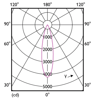
Light Distribution Diagram - RS280 G2 RC Rd D75 11W 40K 24D
