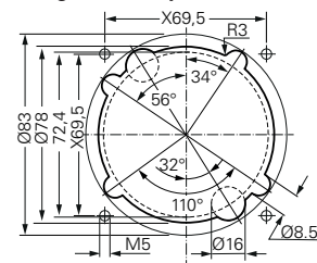
Assembly dimensions flange socket X = fixing dimensions
