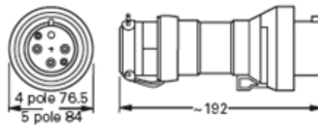
Plug 4/5-pole
