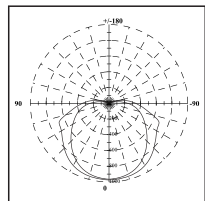
2x58W Photometric
