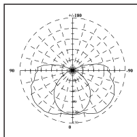
1x18W Photometric
