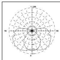
1x36W Photometric
