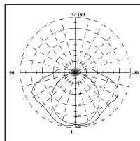
2x18W Photometric
