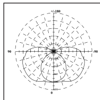
1x58W Photometric
