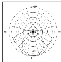
2x36W Photometric
