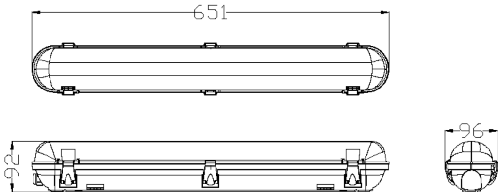
Dampproof Housing 600 1XLAMP & 06x1
