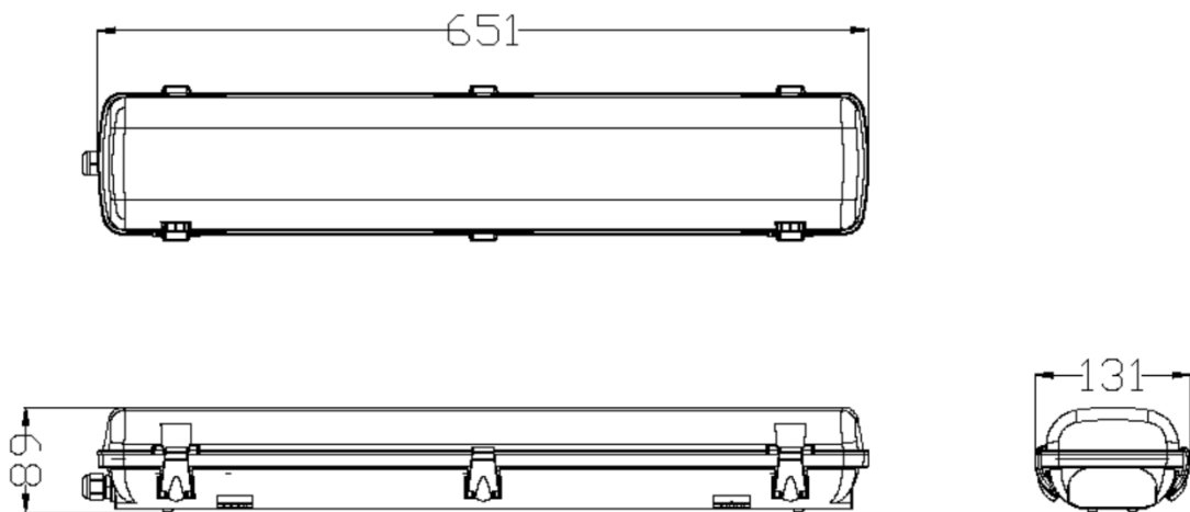
Dampproof Housing 600 2XLAMP & 06x2
