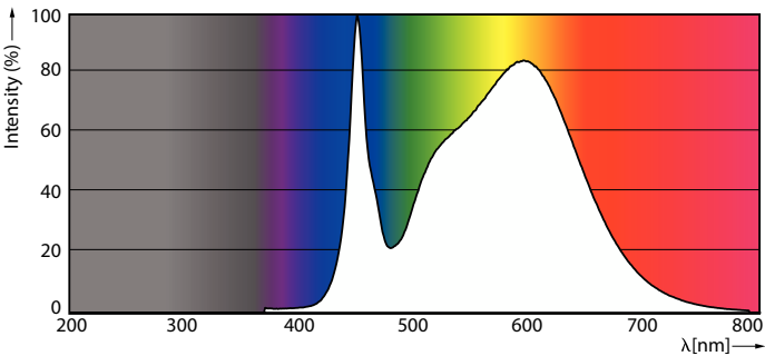
Spectral Power Distribution Colour - MAS LEDtube 1200mm HO 13W840 T8
