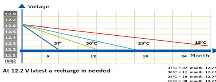
Voltage vs Discharge Time Graph
