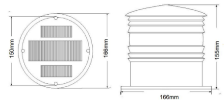
Dimension Drawings
