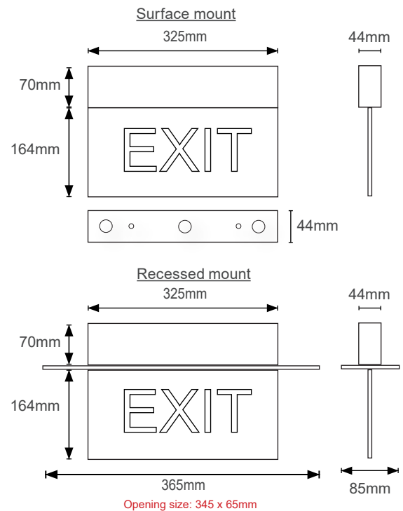
Recess plate REC160
