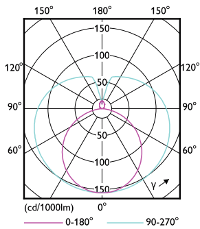
Light Distribution Diagram - CorePro LEDtube 1200mm 16W 865 VVW T8
